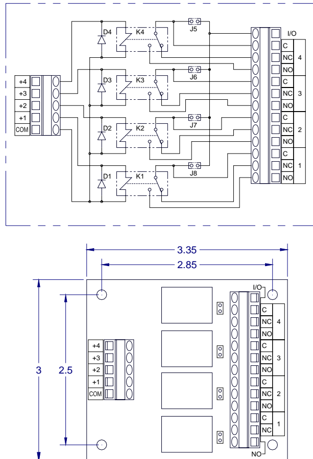
Figure 1 Auxiliary Alarm Relay Board
