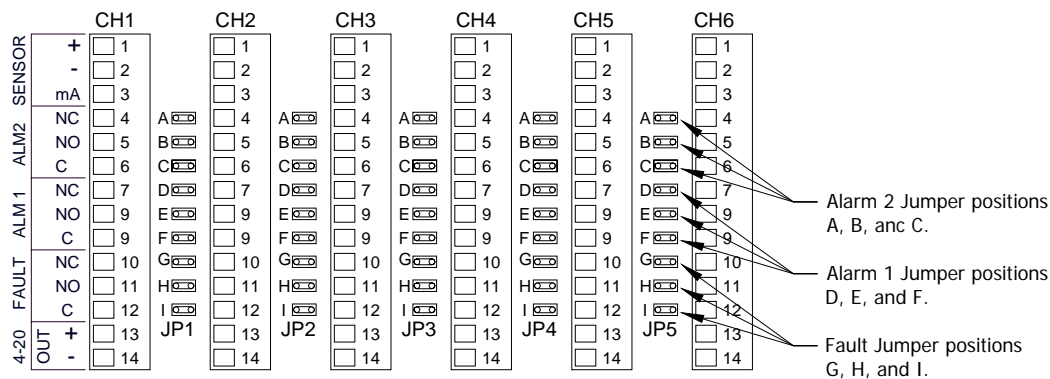
Figure 5 Backplane Configuration Jumpers
